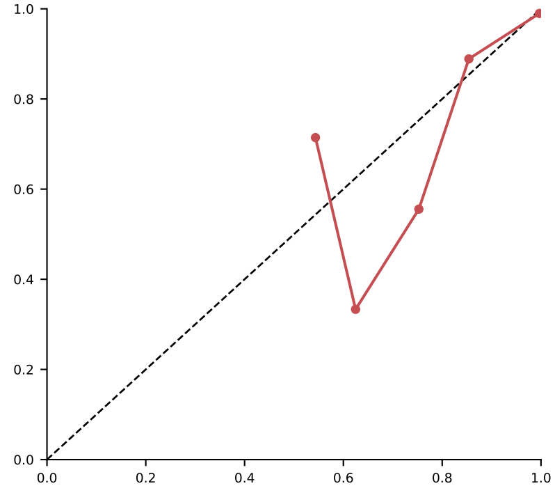
Has_RBC ECE=0.013, n=811
